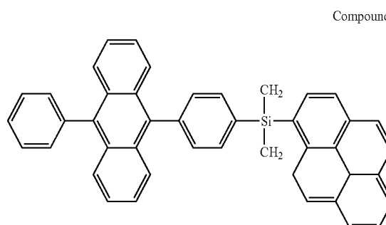
Compound 22
