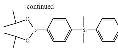
Compound 2-1
